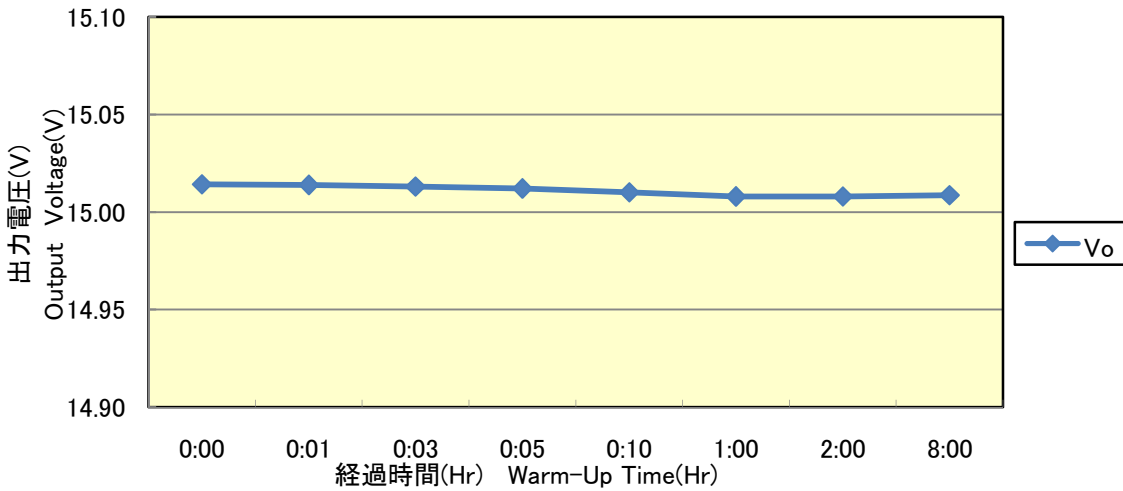
図7 経時ドリフト特性 Fig.7 Warm-Up Drift Characteristics
