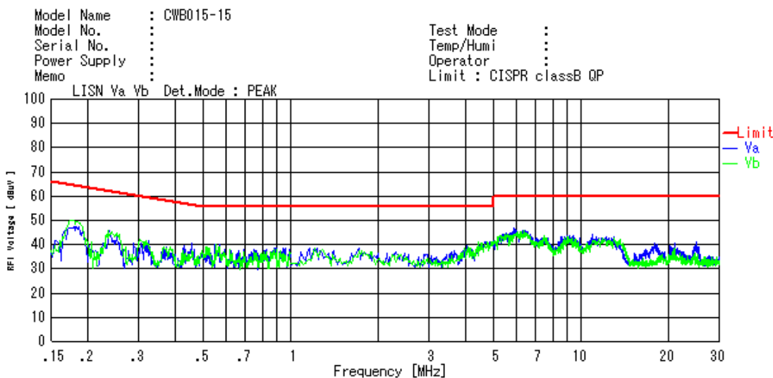
図19 雑音端子電圧 Fig.19 Conduction Noise Waveform
