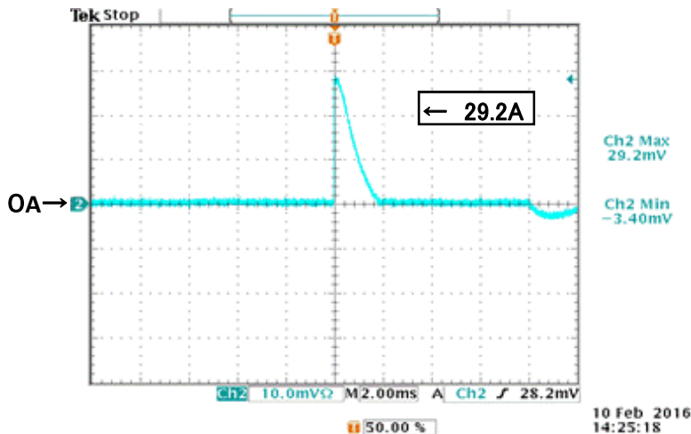
图17 突入電流波形 Fig.17 Inrush Current Waveform
