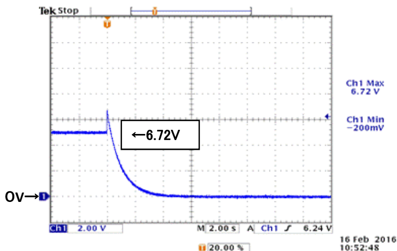
图18 過電圧波形 Fig.18 Over Voltage Waveform
