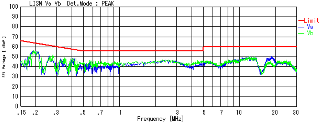
図20 雑音端子電圧 Fig.20 Conduction Noise Waveform
