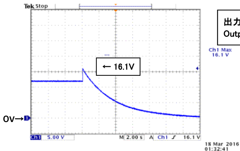
図18 過電圧波形 Fig.18 Over Voltage Waveform
