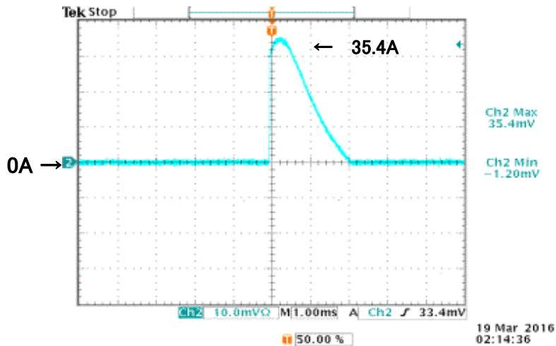
図17 突入電流波形 Fig.17 Inrush Current Waveform
