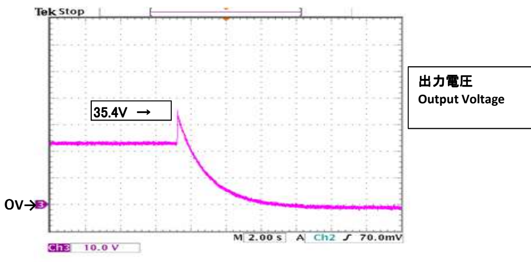
図18 過電圧波形 Fig.18 Over Voltage Waveform
