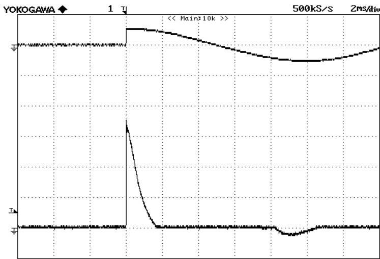
図16 突入電流波形 Fig.16 Inrush Current Waveform
