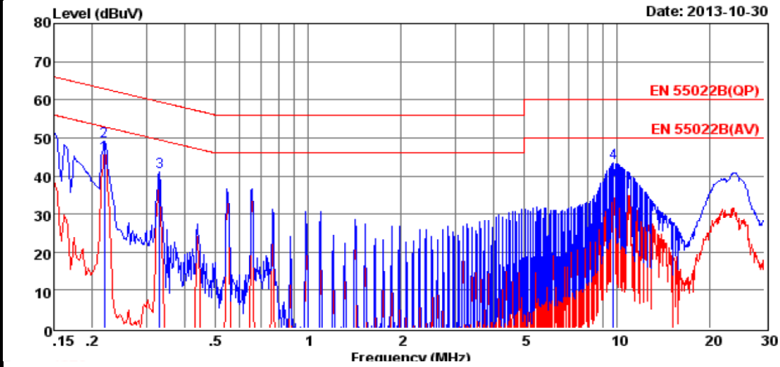
図18 雑音端子電圧波形 Fig.18 Conduction Noise Waveform
