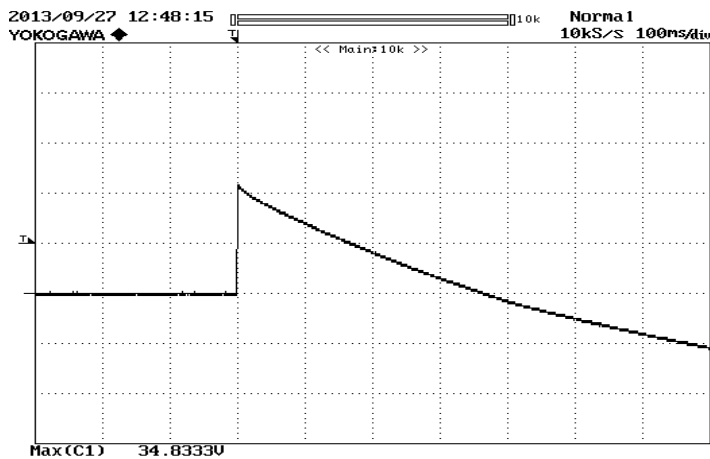
図17 過電圧波形 Fig.17 Over Voltage Waveform
