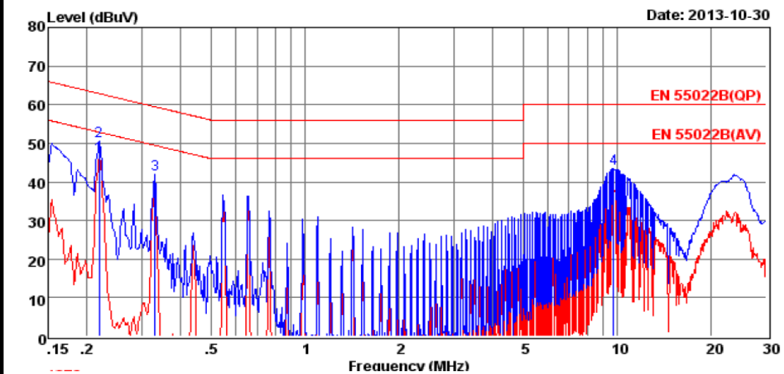
図19 雑音端子電圧 Fig.19 Conduction Noise Waveform
